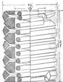
Fig. 3934. Harvey Friction Draft Spring. Frost Ry. Supply Co.
